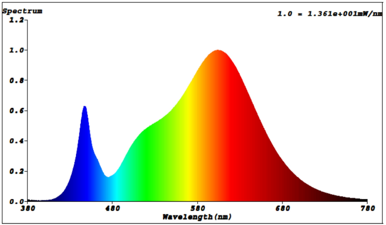
PL-0332GA at 3000K
