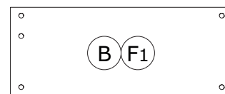
FS4445 694x279x16mm
