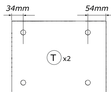
TR2575 218x280x16mm
