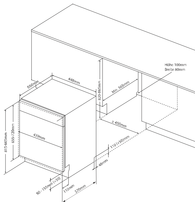
GS4503 offen
