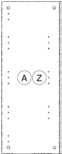
FI10419 836x335x16mm
