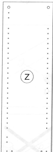
FI8505 968x327x18mm
