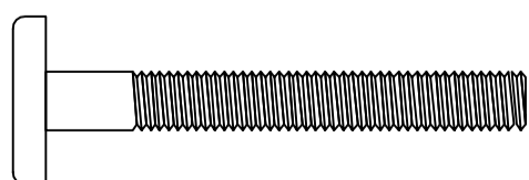
Boulon M8x60
