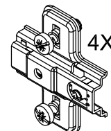
4X FFBMP2020
