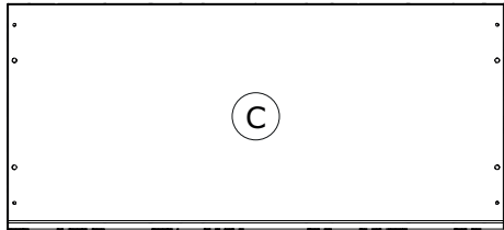
CA04309 893x405x22mm
