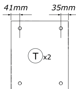
TR2577 325x268x16mm
